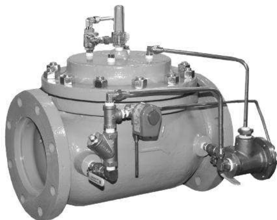
▲ Electric / Hydraulic Deluge Valve
