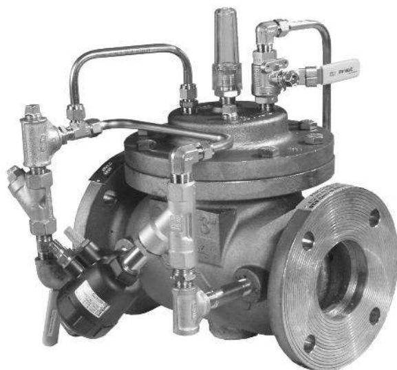
▲ Pneumatic / Hydraulic Deluge Valve
