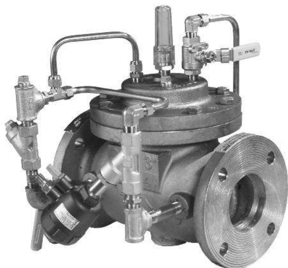
▲ Pneumatic / Hydraulic Deluge Valve
