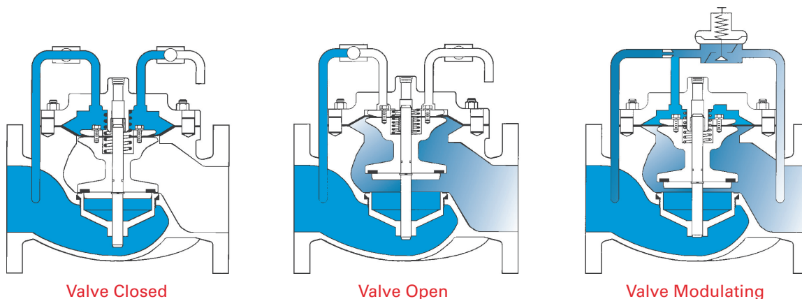
Valve Closed
