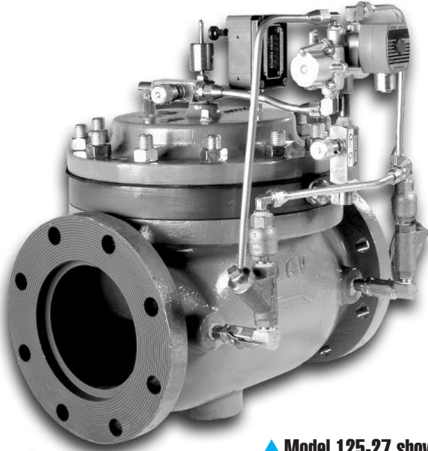
▲ Model 125-27 shown
