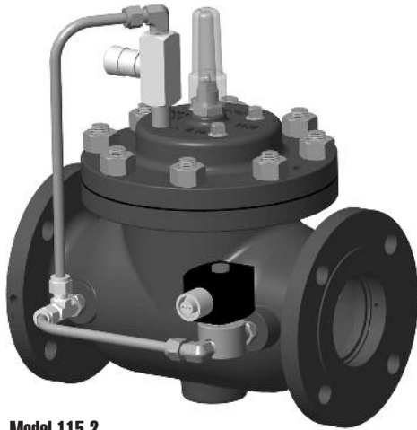
▲ Model 115-2
