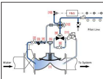
Manually Actuated &amp; Pressure Reducing
