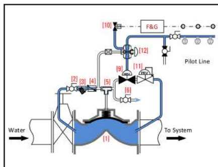
Manually Actuated (Standard)
