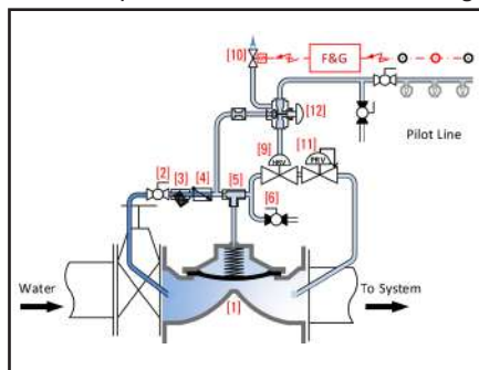
Electrically Actuated &amp; Pressure Reducing
