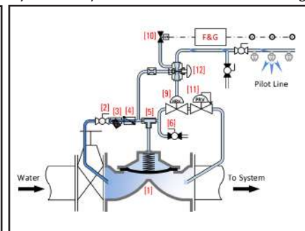
Hydraulically Actuated &amp; Pressure Reducing
