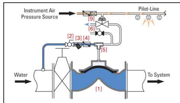
Pneumatically Actuated
