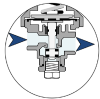
De-pressurized Sensor Line / Command
