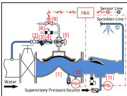
Sprinkler Burst &amp; Sensor Line Activated
