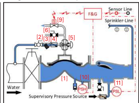
Sensor Line Activated - Pipeline Filled (Single-Interlock Only)
