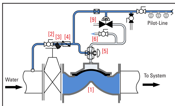
Manually Actuated
