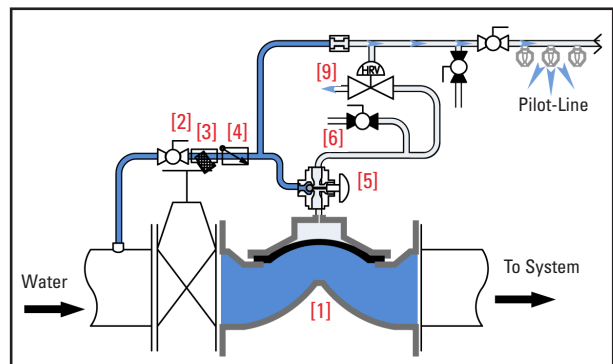
Hydraulically Actuated
