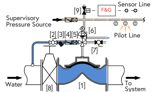
Pneumatically Actuated
