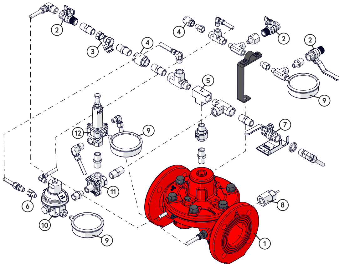
General representation of valve.
